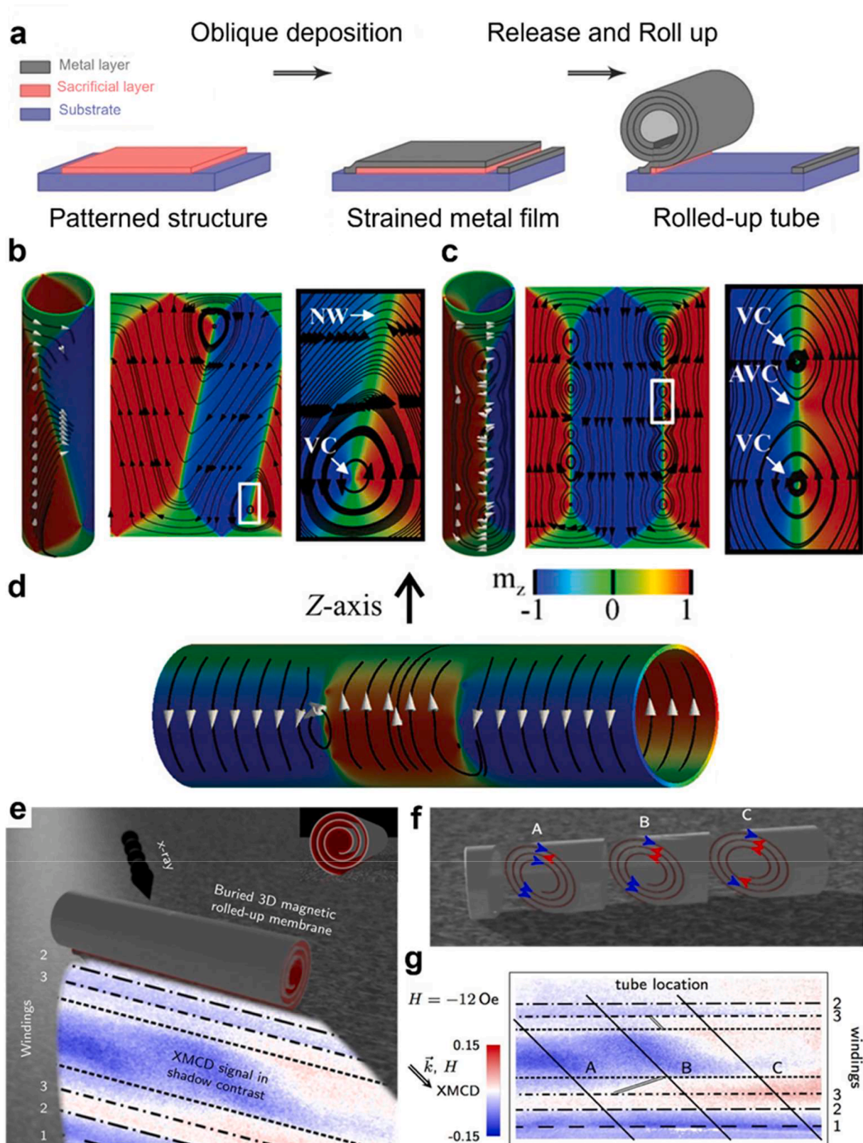
Fig. 5. Magnetic Domain Characteristics in Rolled-up Architectures. a, Schematic illustration of the device used for investigating magnetic domain structures in rolled-up tubular architectures. b, Random distribution and c, A predefined two-domain state of rolled-up permalloy domain structures. d, Domain structures of rolled-up nickel films. e, XMCD characterization of magnetic materials within tubular structures. f, XMCD images of different windings in the rolled-up system under varying external magnetic fields. g, Corresponding magnetic domain patterns. Reproduced with permission. Copyright © 2013, Wiley-VCH. Copyright © 2014, American Chemical Society.
