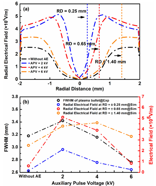
FIG. 5. (a) The radial distribution of radial electrical field in discharge without AE (black) and discharge with APV = 2.0 kV (blue), 4.0 kV (red), and 6.0 kV (orange); (b) the FWHM of plasma bullets and radial electrical field obtained from RD = \pm 0.25 mm (blue), \pm 0.65 mm (red), and \pm 1.40 mm (orange) in discharge without AE and APV = 2.0, 4.0, and 6.0 kV.
