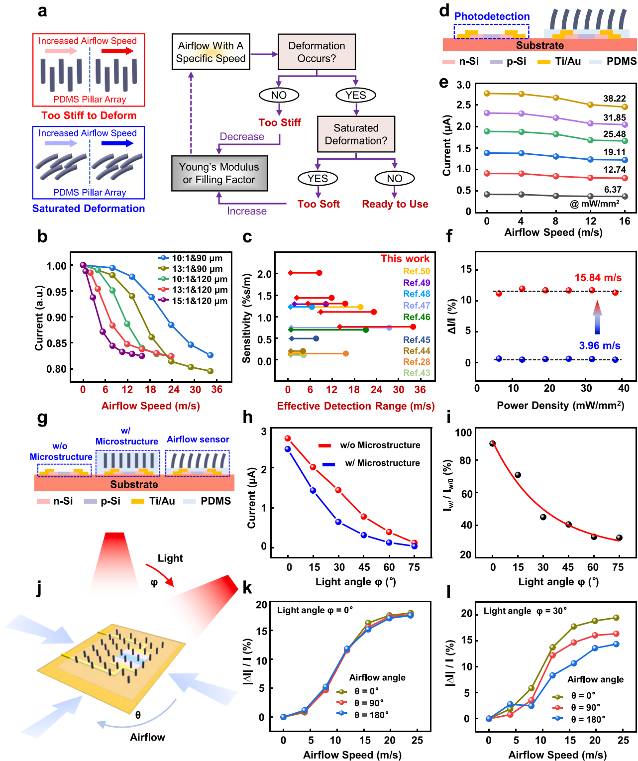
Fig. 4. Characterization and optimization of the airflow sensor. (a) Typical issues (left) and optimization flow chart (right) of the airflow sensor. (b) Photocurrent variations with the airflow speed obtained from different optoelectromechanical sensors, of which the black PDMS pillars have different weight ratios of base to crosslinker and neighboring distances (i.e., filling factors). (c) Comparisons in effective detection range and sensitivity of the demonstrated sensor with those of other previous reports [28,43–50]. (d) Schematic of the simultaneous operation of photodetection and airflow sensing. (e) Photocurrents obtained from the airflow sensor varying with the airflow speed under different light power intensities. (f) Changes in photocurrent varying with the light power density for two typical airflow speeds. The change in photocurrent exhibits negligible relationship with the incident light power density, but is strongly determined by the airflow speed. (g) Schematic of the simultaneous operation of light incident direction recognition and airflow sensing. (h) Photocurrents obtained from the photodetectors with and without microstructured layer varying with the light illumination angle \phi . (i) The ratio of photocurrent obtained from the photodetectors with and without microstructured layer varying with the light illumination angle \phi . (j) Schematic of airflow sensing under different illumination angles ( \phi ) and airflow angles ( \theta ). Airflow speed sensing under different airflow angles: (k) illumination angle \phi = 0^\circ ; (l) illumination angle \phi = 30^\circ .
