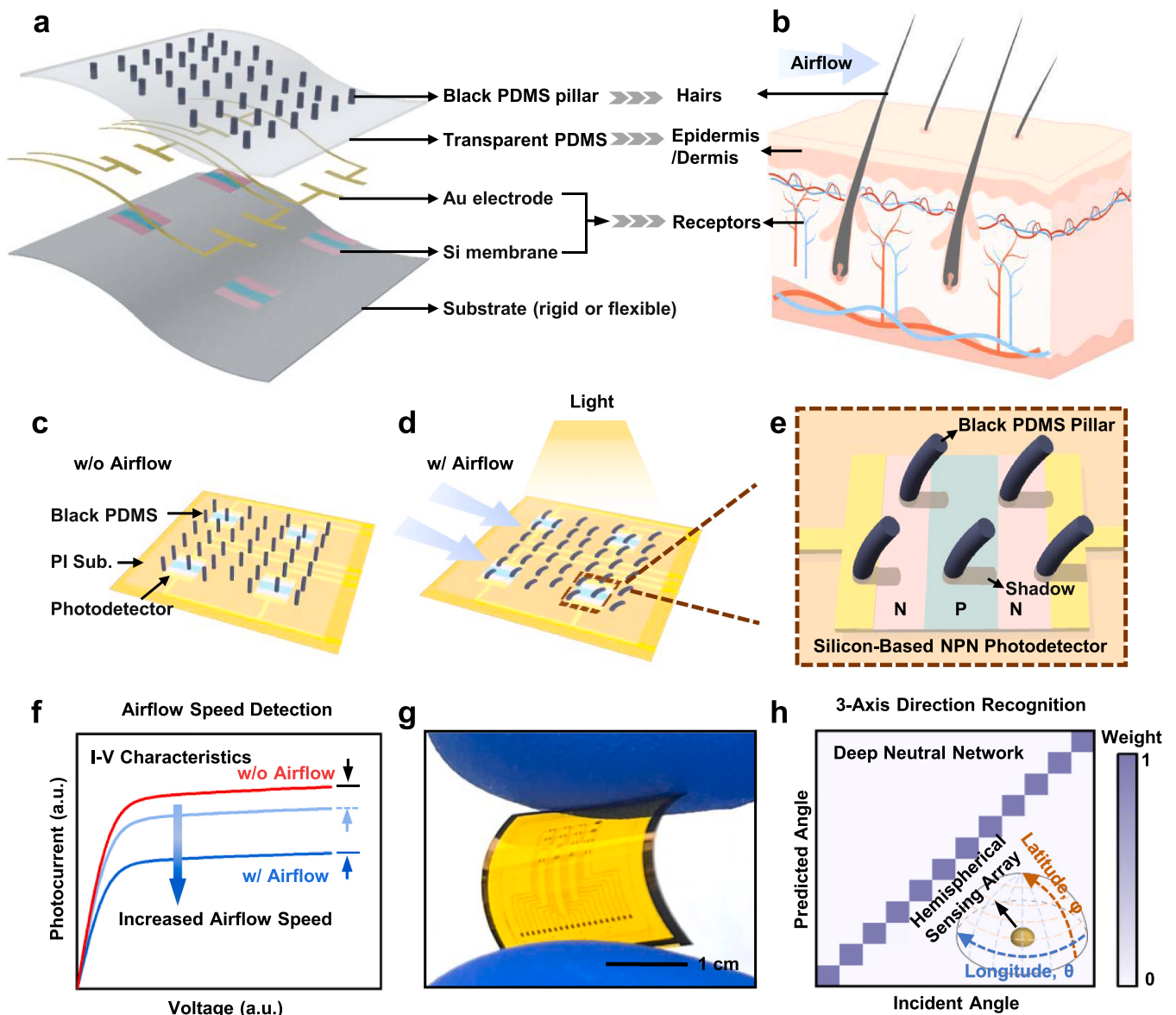
Fig. 1. Key materials and working principle of the optoelectromechanical airflow sensor. (a) Exploded Schematic of key materials and architectures. (b) Schematic diagram of the human skin sensor with hairs, epidermis/dermis, and receptors. Schematics of an airflow sensor array without (c) and with (d) airflow. (e) A magnified diagram of the airflow sensor with airflow, which blows black PDMS pillars to deform. (f) Conceptual variations of photocurrents without (red curve) and with (blue curves) airflow. (g) Optical image of silicon-based photodetector array on flexible substrate. (h) Conceptual 3-axis direction recognition by a hemispherical sensing array through the deep neutral network. The inset shows the configuration for 3-axis airflow sensing, including the inner hemispherical sensing array, an outer shell for the airflow control, and the 3-axis direction referred to the latitude, \phi and the longitude, \theta .
